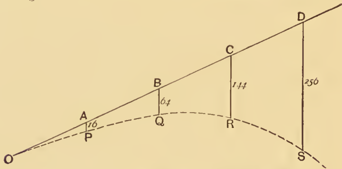
FIG. 57.—Parabolic orbit of a projectile (cf. p. 82).
